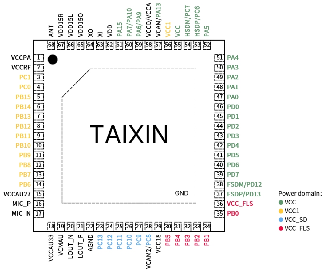
Figure 1-4-1: TXW828-C08FL QFN68 Package Pin Layout
